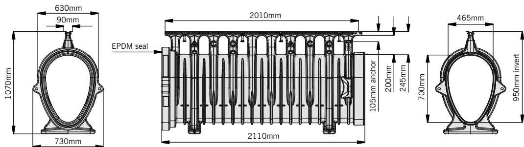
ACO Qmax® 700 with ACO Q-Flow galvanised steel edge rail
