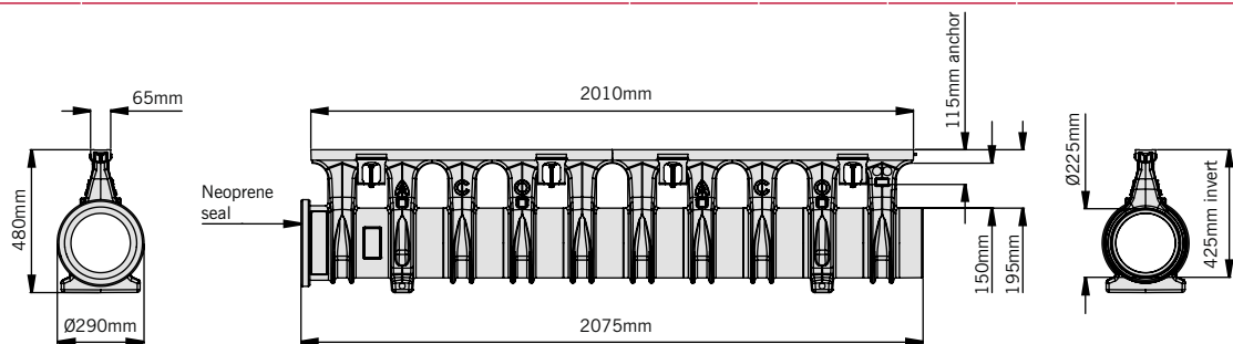
ACO Qmax® 225 with ACO Q-Guard ductile iron edge rail
